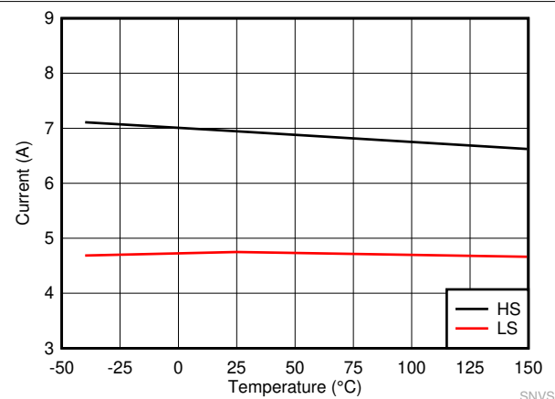
图 8-4. LM62440-Q1 High-side and Low-side Current Limits
