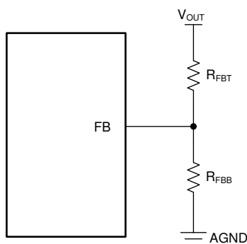
图 9-17. Setting Output Voltage of Adjustable Versions
