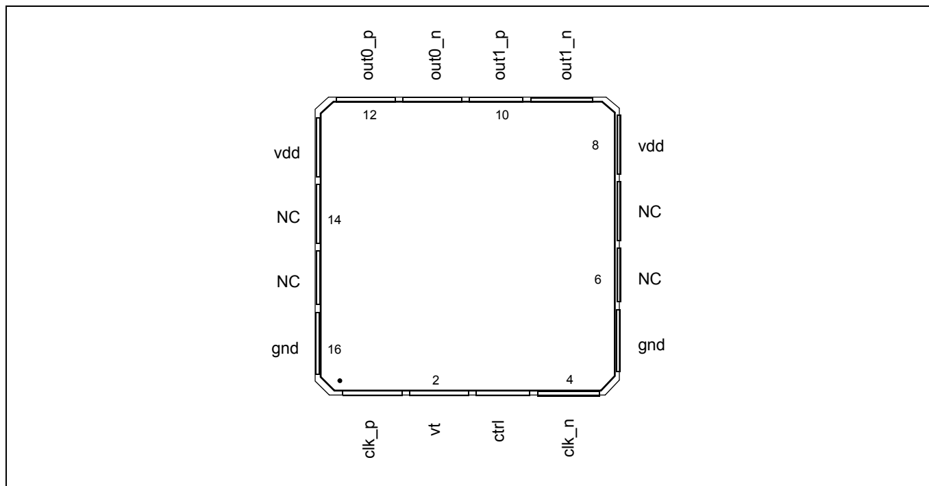
Figure 2 - Pin Connections
