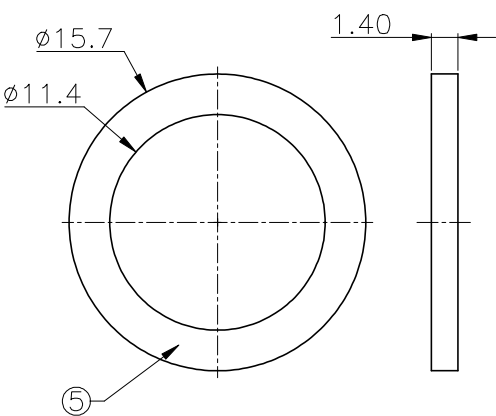
WASHER
