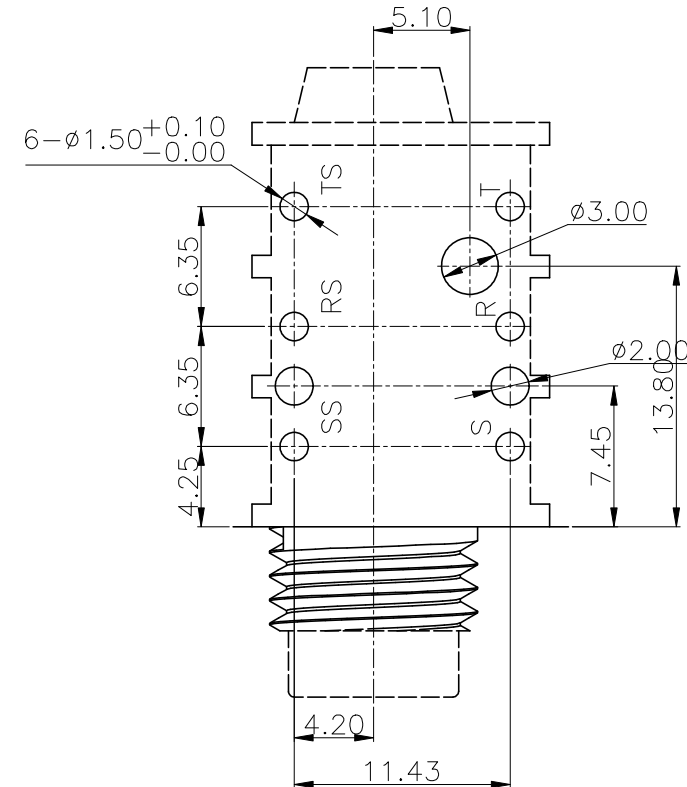
RECOMMENDED PCB LAYOUT (TOP VIEW TOLERANCE:±0.05)
