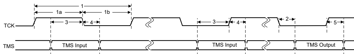
Figure 6-32. cJTAG Timing
