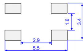
推荐焊盘 Recommended Land Pattern
