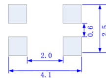
推荐焊盘 Recommended Land Pattern
