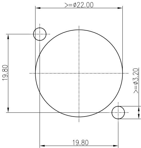
CHASSIS MOUNTING HOLES PANEL CUT OUT (front side)
