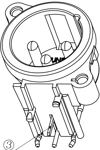
3D VIEW
