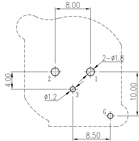
P.C.B. LAYOUT(TOLERANCE:±0.1) (TOP VIEW)
