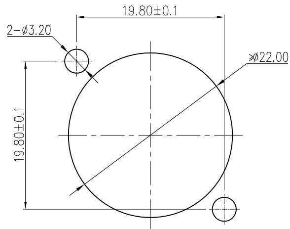
CHASSIS MOUNTING HOLES PANEL CUT OUT (front side)
