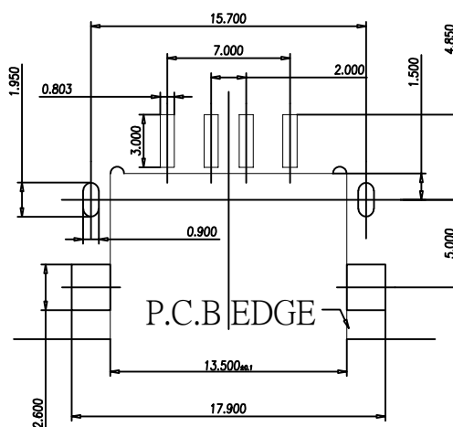
RECOMMENDED P.C.B. PATTERN LAYOUT
