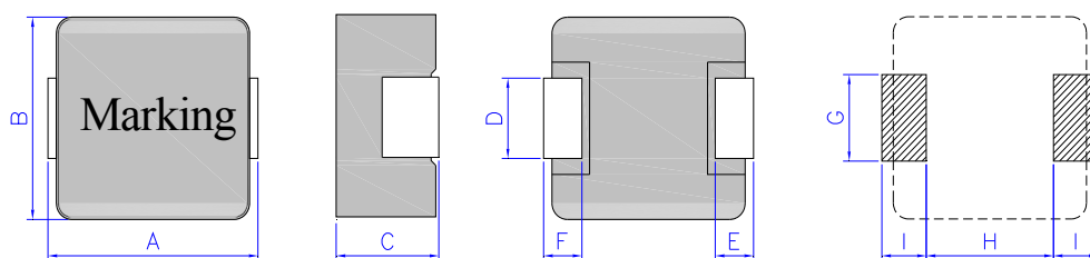
RECOMMENDED LAND PATTERNS
