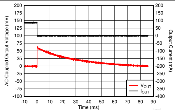
图 6-18. I_{OUT} Transient From 100 mA to 0 mA
