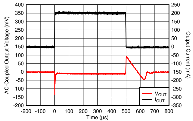
图 6-14. I_{OUT} Transient From 1 mA to 200 mA
