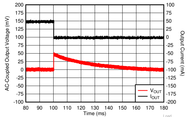
图 6-16. I_{OUT} Transient From 50 mA to 0 mA
