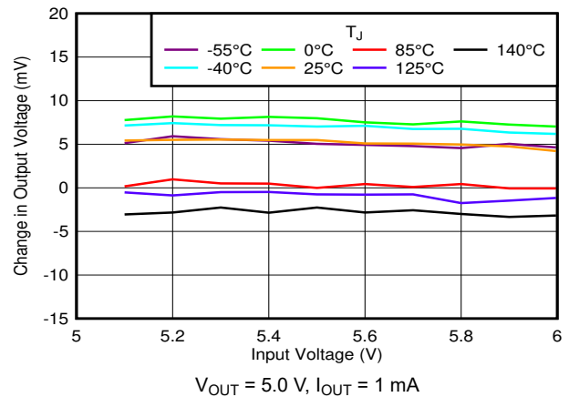
图 6-28. Line Regulation vs V_{IN} and Temperature
