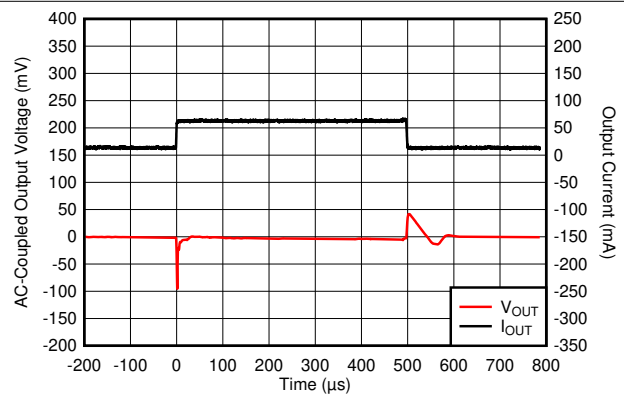
图 6-12. I_{OUT} Transient From 1 mA to 50 mA
