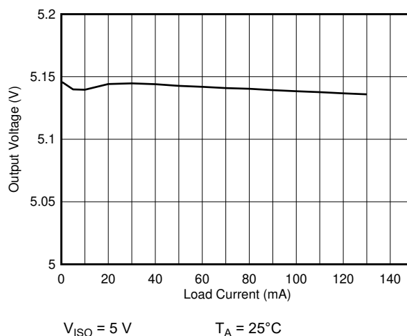
图 7-4. Isolated Supply Voltage ( V_{ISO} ) vs Load Current ( I_{ISO} )
