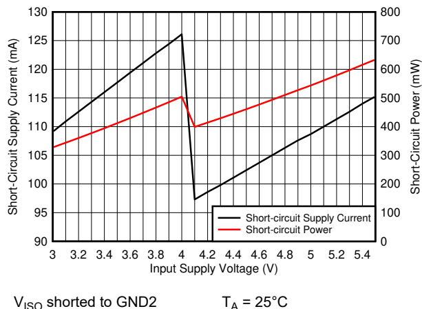
图 7-10. Short-Circuit Supply Current ( I_{CC} ) and Power ( P ) vs Supply Voltage ( V_{CC} )
