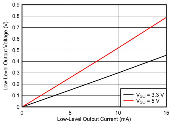
图 7-16. Low-Level Output Voltage vs Low-Level Output Current
