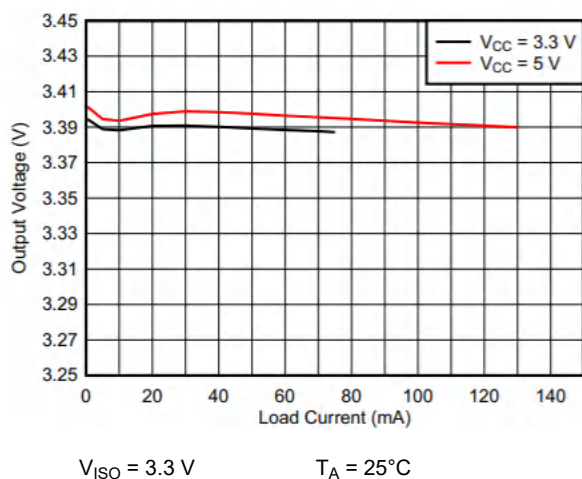
图 7-3. Isolated Supply Voltage ( V_{ISO} ) vs Load Current ( I_{ISO} )
