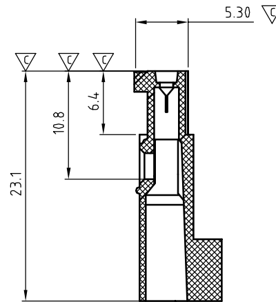
Section P-P
