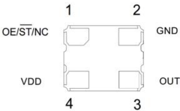
Pin Assignments
