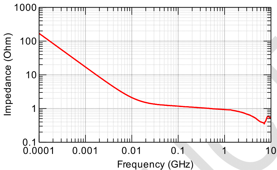
Figure 2 Impedance characteristic versus Frequency in shunt mode
