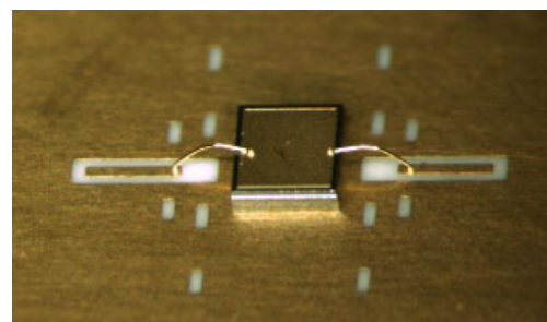
Figure 4 – micro picture of mounted 0202 WLSC/WBSC
