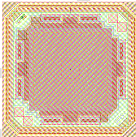
Figure 6 – Layout view
