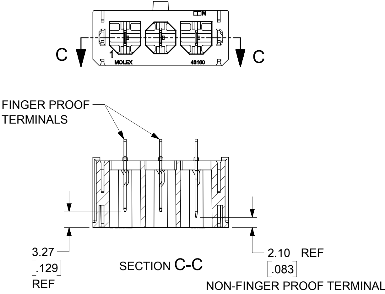
HEADER WITH OPTIONAL FINGER PROOF TERMINAL 43160-9002 SHOWN
