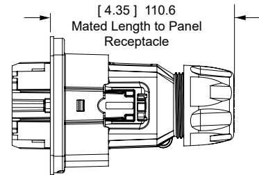
Mated View
