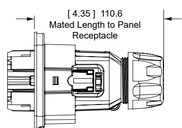
Mated View
