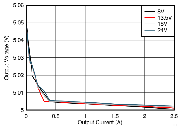
LM63625 V_{OUT} = 5V f_{SW} = 2100 kHz (自动)
