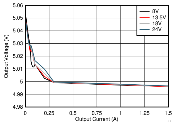
LM63615 V_{OUT} = 5V f_{SW} = 2100 kHz (自动)
