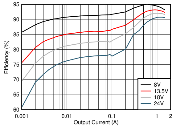
LM63615 V_{OUT} = 3.3V f_{SW} = 400 kHz (自动)
