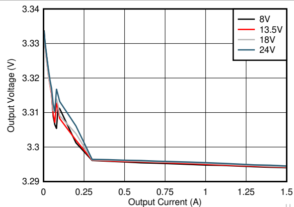
A. LM63615 V_{OUT} = 3.3V f_{SW} = 2100 kHz (自动)
