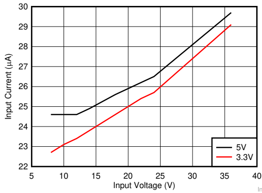
LM63625 I_{OUT} = 0A f_{SW} = 2100kHz (自动)
