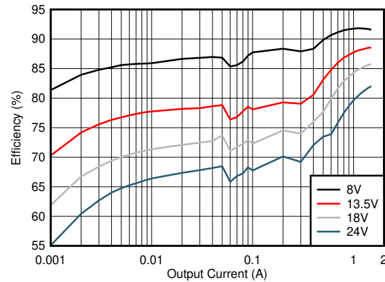
LM63615 V_{OUT} = 3.3V f_{SW} = 2100 kHz (自动)
