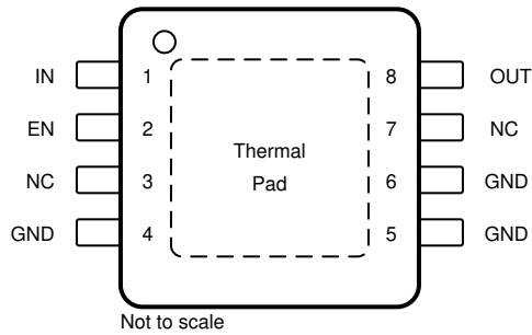
图 5-1. DGN Package, 8-Pin HVSSOP (Top View)
