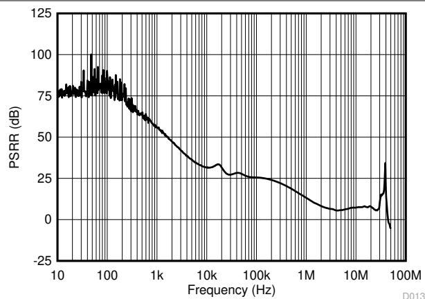
I_{OUT} = 100\text{ mA} 图 6-13. PSRR vs Frequency
