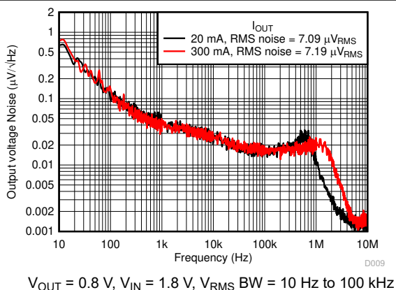
图 5-71. Noise vs Frequency and I_{OUT}
