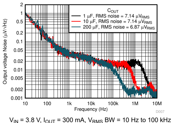
图 5-69. Noise vs Frequency and C_{OUT}
