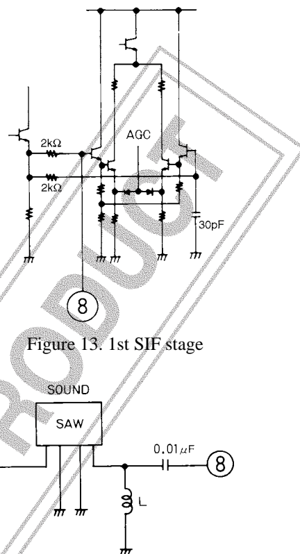
Figure 14. SAW filter matching
