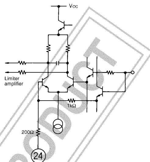
Figure 29. SIF stage input circuit
