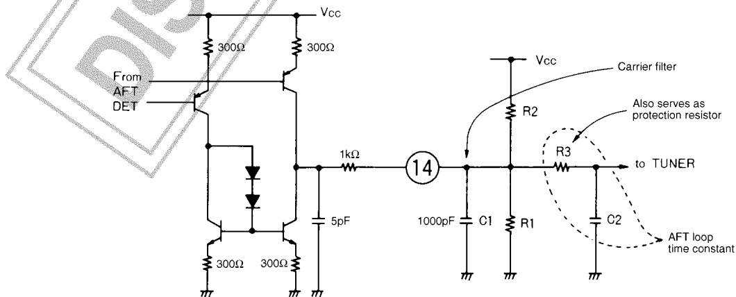
Figure 19. AFT loop time constant
