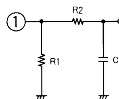
Figure 6. RC de-emphasis circuit
