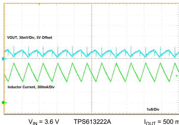
图 8-12. Switching Waveform at Heavy Load
