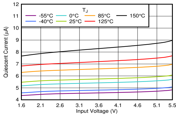
图 5-37. I_{GND} vs V_{IN} in the Dropout Region
