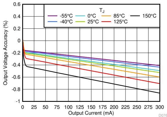
图 5-13. Output Voltage Accuracy vs I_{OUT}
