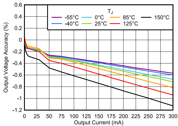
图 5-13. Output Voltage Accuracy vs I_{OUT}
