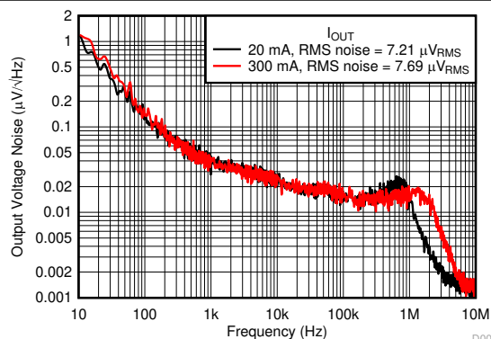
图 5-70. Noise vs Frequency and I_{OUT}
