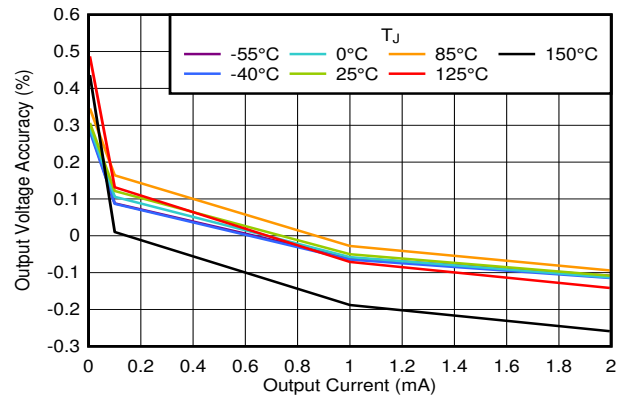
图 5-14. Output Voltage Accuracy vs I_{OUT}
