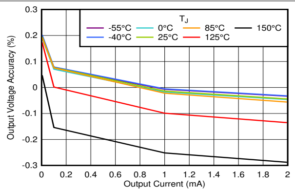
图 5-16. Output Voltage Accuracy vs I_{OUT}
