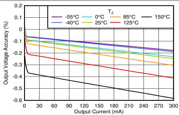
图 5-15. Output Voltage Accuracy vs I_{OUT}
