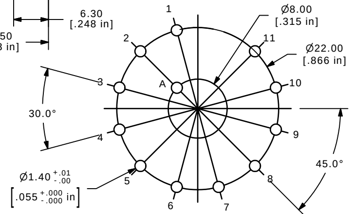
P.C.B MOUNTING LAYOUT
