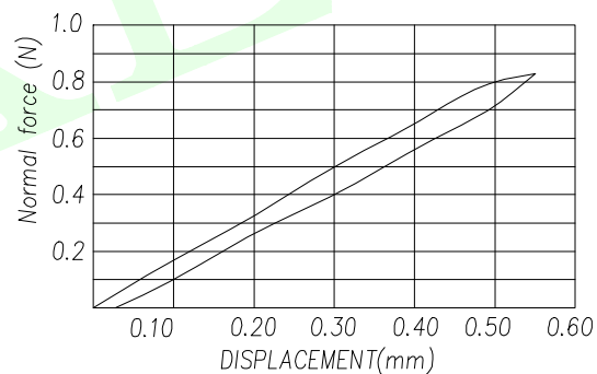
Nano Sim card Contact NF-Deflection Curve
