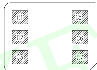
NANO SIM CARD ELECTRICAL
