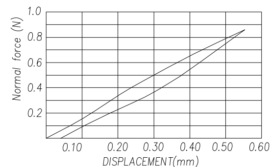
Micro SD Card Contact NF-Deflection Curve
