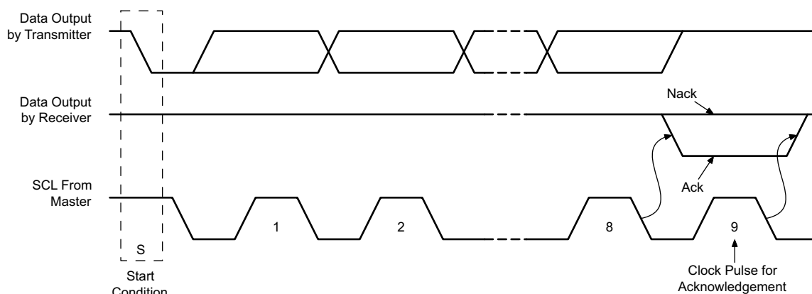
图 8-24. I²C Acknowledgment
