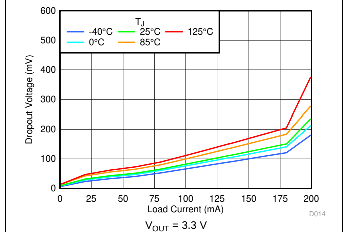
图 22. Dropout vs I_{OUT} and Temperature
