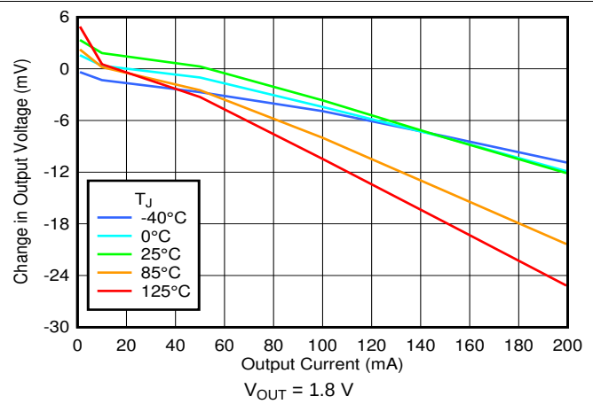
图 28. Load Regulation vs I_{OUT} and Temperature
