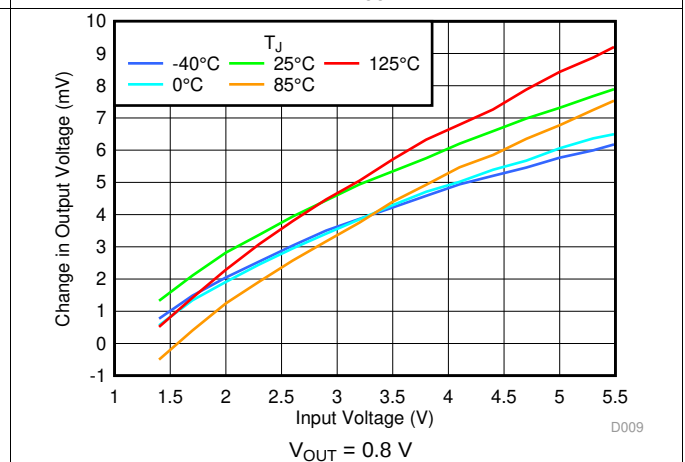
图 24. Line Regulation V_{IN} and Temperature
