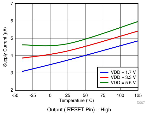
图 7-9. Supply Current vs Temperature
