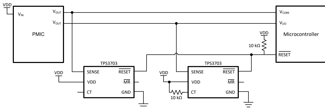
图 9-6. Two TPS3703 Monitoring Two Microcontroller Power Rails
