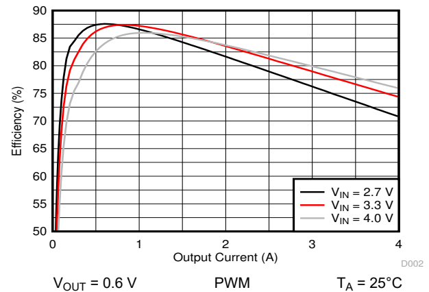
图 10-11. Efficiency versus Output Current
