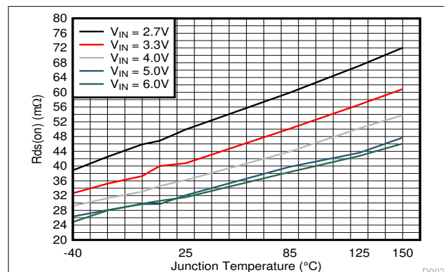
图 7-1. R_{ds(on)} of High-side Switch
