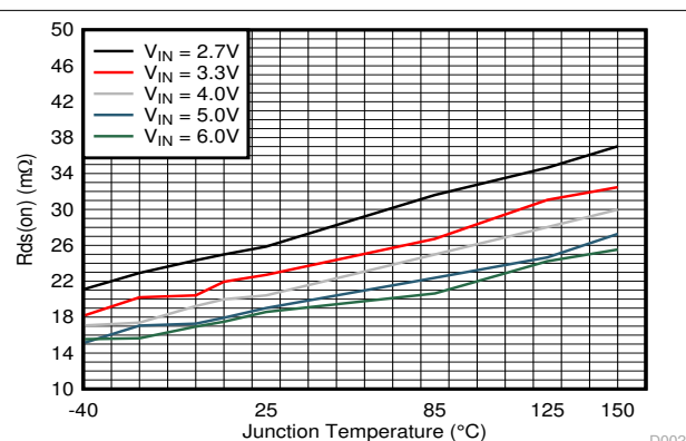
图 7-2. R_{ds(on)} of Low-side Switch
