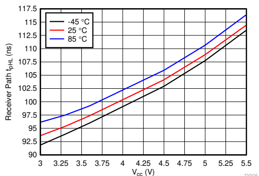
图 5-3. Receiver path high-to-low propagation delay, C_L = 150\text{pF} (RGT package)
