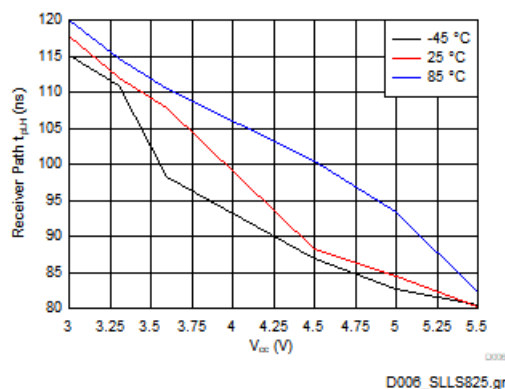
图 5-4. Receiver path low-to-high propagation delay, C_L = 150\text{pF} (RGT package)
