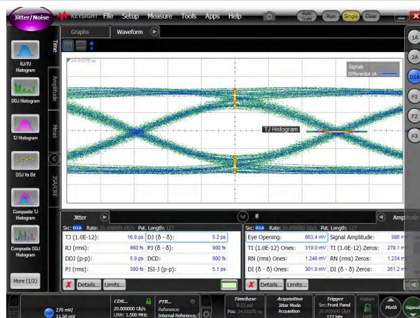
图 5-6. Jitter Decomposition of 20Gbps PRBS-7 Signals in TI Evaluation Board Through a Typical TMUXHS4412 Channels
