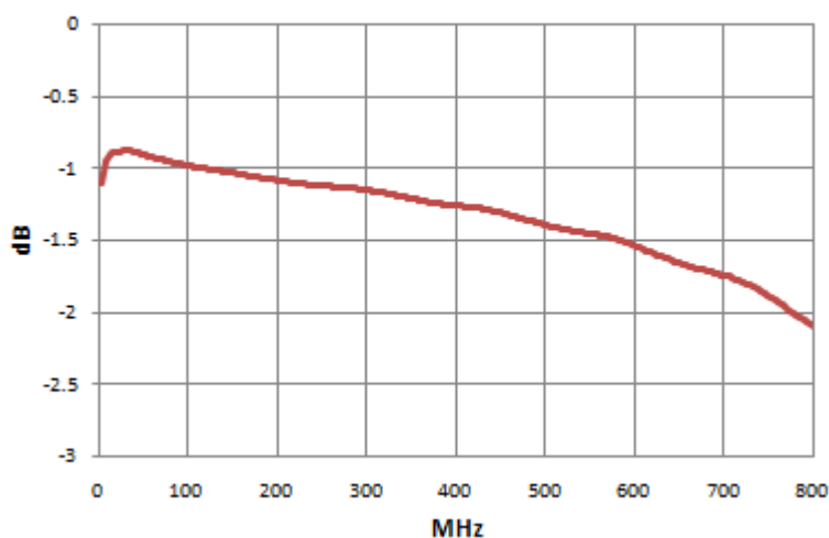
Insertion Loss 6-1
