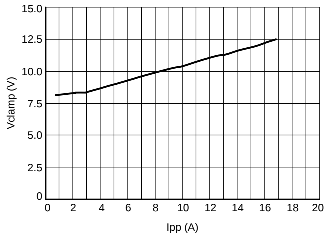
Figure 2. Clamping Voltage vs. Peak Pulse Current (t p = 2/10 μs, R = 8 Ω)
