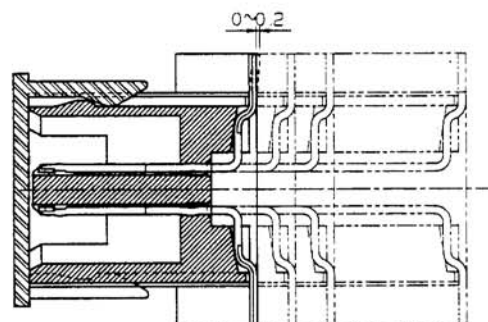
SECT. X-X
