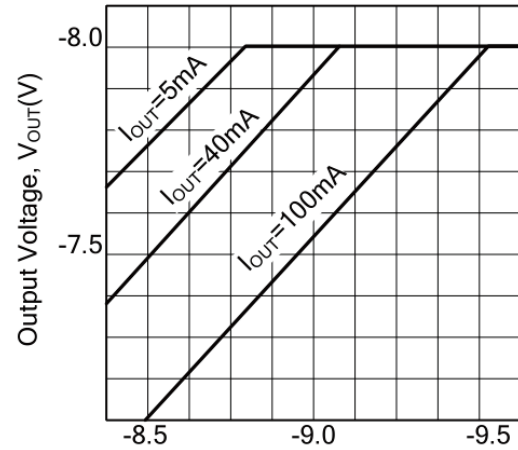
UTC79L08 Dropout Characteristics ( T_J=25^\circ\text{C} )
