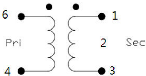
SCHEMATIC
