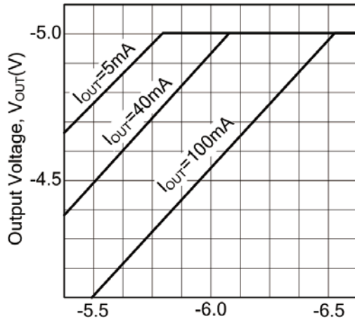
UTC79L05 Dropout Characteristics ( T_J=25^\circ\text{C} )
