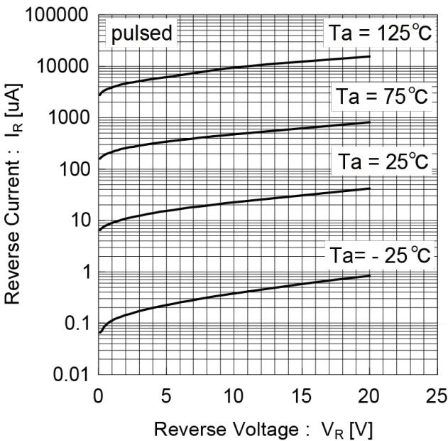
Fig.12 Reverse Current vs. Reverse Voltage
