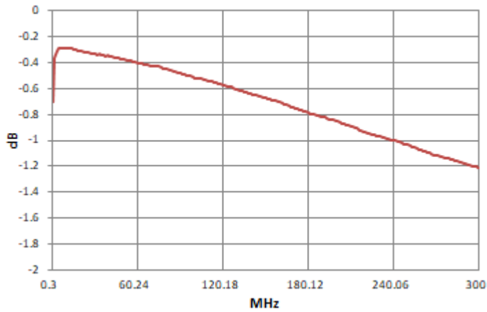
Insertion Loss
