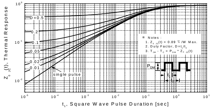
Figure 11-1. Transient Thermal Response Curve for FQP4N90C
