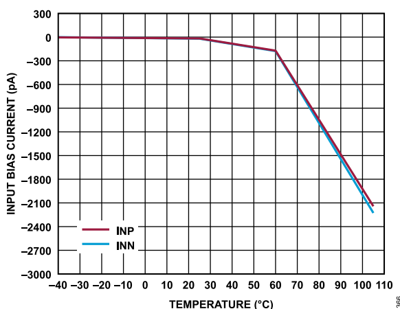
Figure 66. Input Bias Current vs. Temperature
