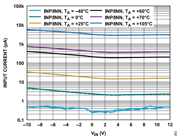
Figure 63. Input Current vs. Input Voltage across Temperature
