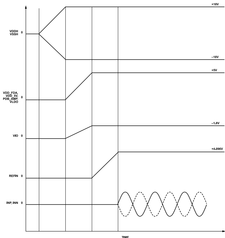
Figure 102. Power Supply Sequence
