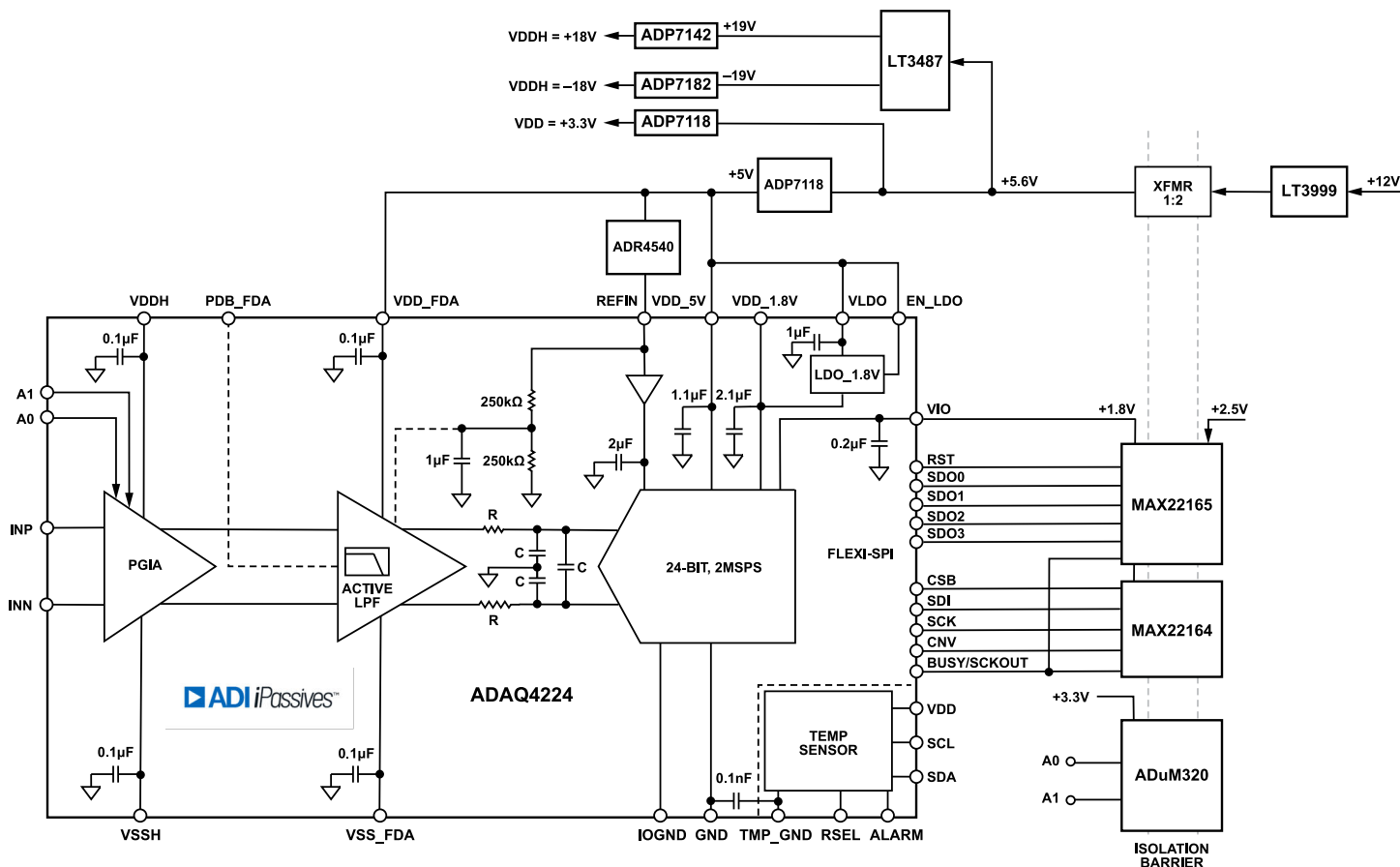
Figure 90. Functional Block Diagram of a Fully Isolated Data-Acquisition System
