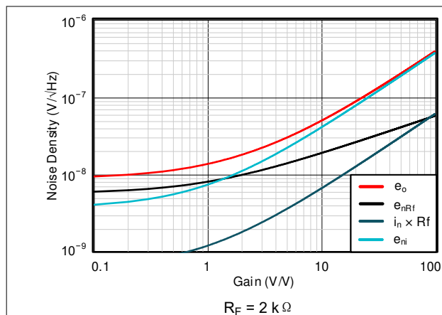
图 9-5. Calculated Noise Densities vs Gain Settings
