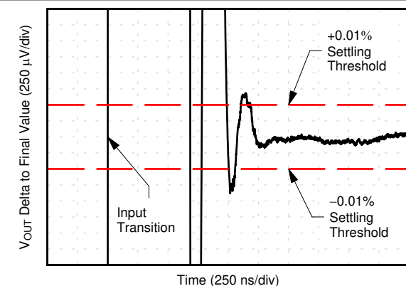
图 6-36. Output Settling Time to \pm 0.01\%
