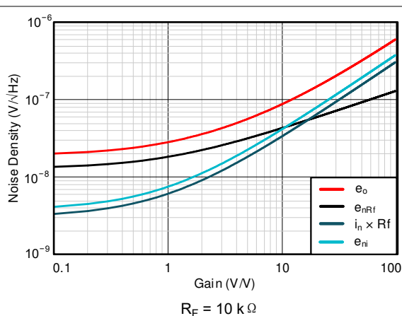
图 9-6. Calculated Noise Densities vs Gain Settings
