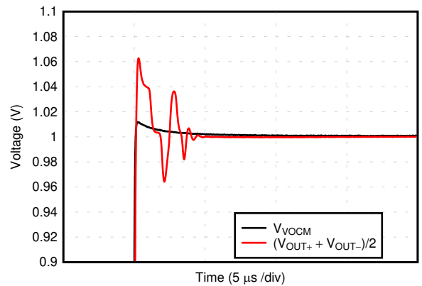
图 6-34. Output Common-Mode Step Response, Rising
