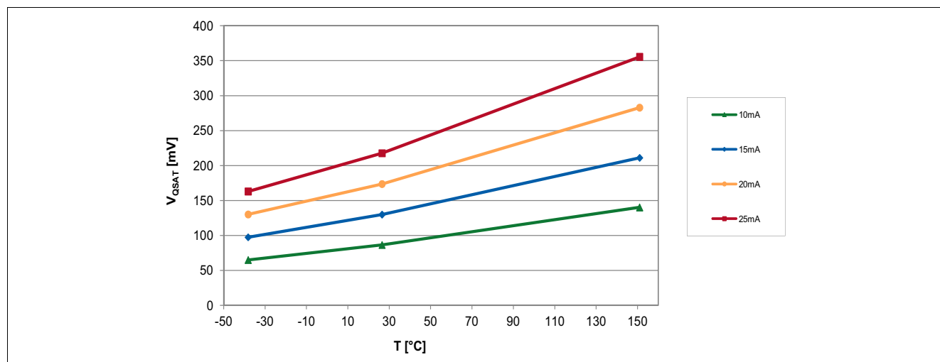
Figure 30 Saturation voltage of the TLV4961-1M over temperature
