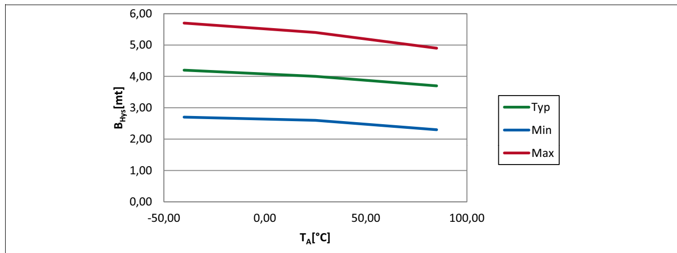
Figure 18 Hysteresis ( B_{Hys} ) of the TLV4961-1M over temperature
