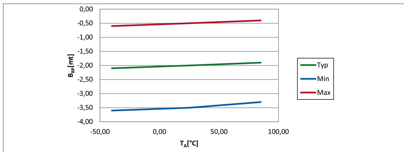
Figure 17 Release point ( B_{RP} ) of the TLV4961-1M over temperature
