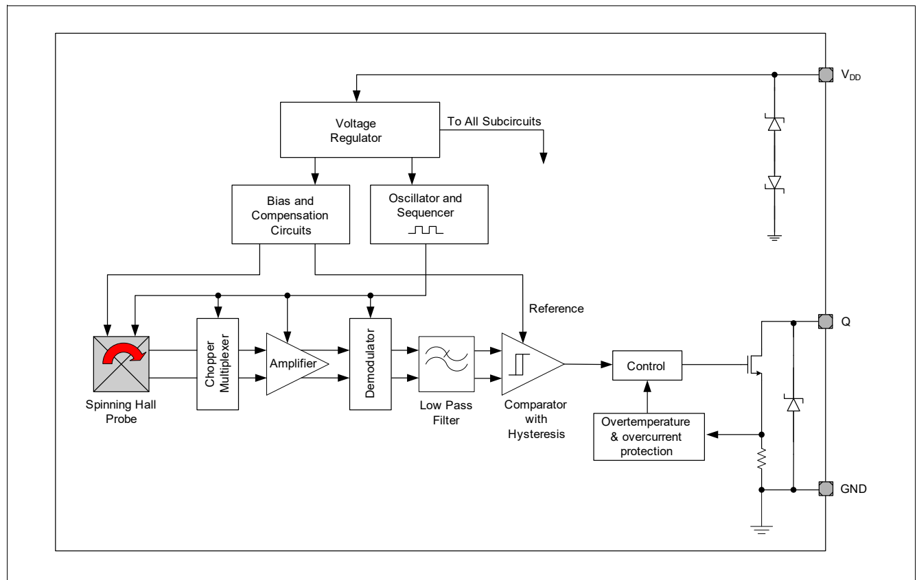
Figure 3 Functional block diagram TLV4961-1M
