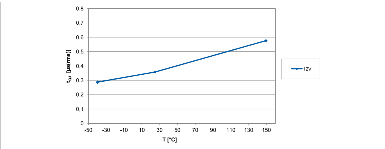
Figure 33 Output signal jitter of the TLV4961-1M over temperature
