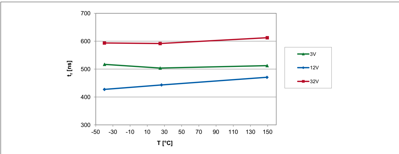
Figure 27 Output rise time of the TLV4961-1M over temperature
