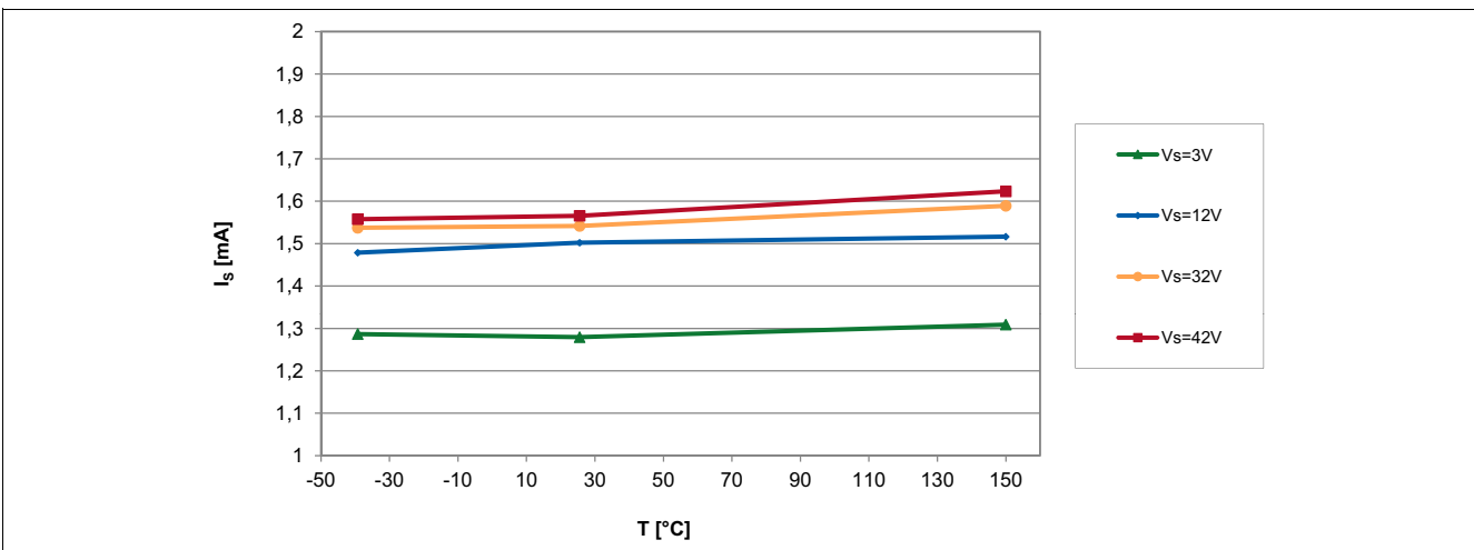
Figure 21 Supply current of the TLV4961-1M over temperature
