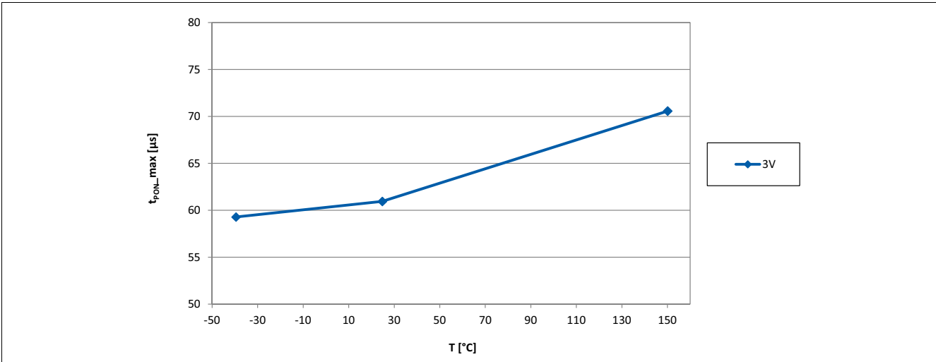
Figure 19 Power on time t_{PON} of the TLV4961-1M over temperature
