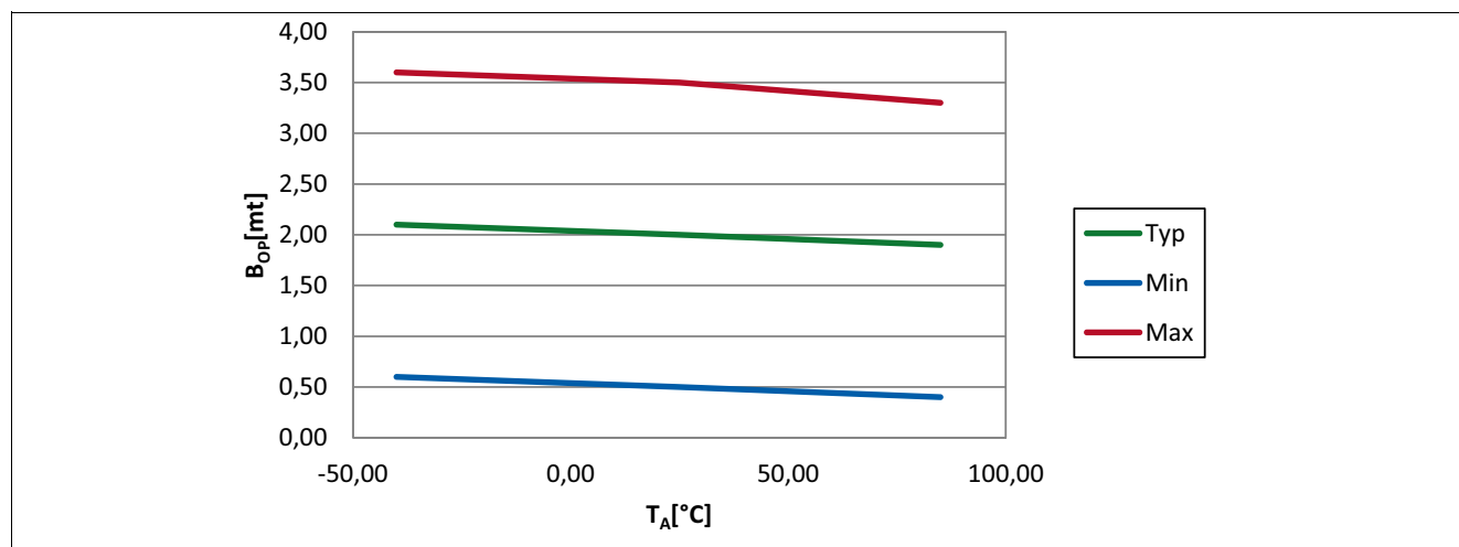
Figure 16 Operating point ( B_{OP} ) of the TLV4961-1M over temperature
