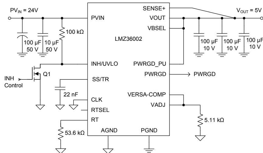
图 37. LMZ36002 Typical Schematic
