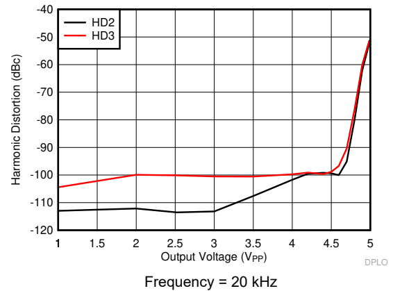
图 7-10. Harmonic Distortion vs Output Voltage
