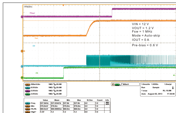
图 29. Pre-Bias Operation
