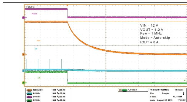
图 25. Shutdown Operation
