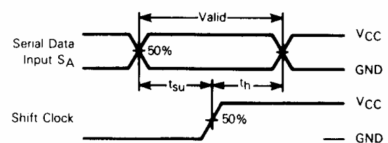
Figure 6. Switching Waveforms
