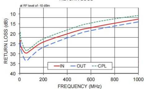
RETURN LOSS
