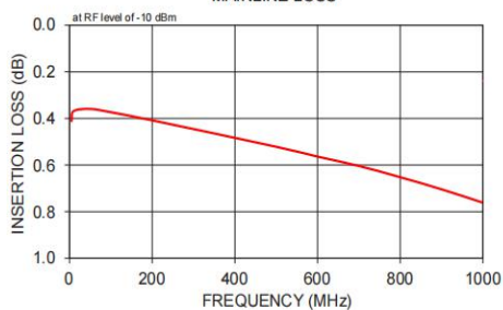
MAINLINE LOSS
