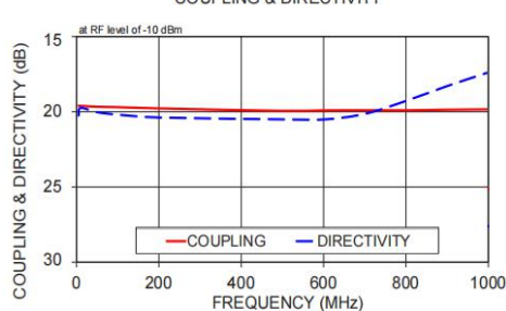
COUPLING & DIRECTIVITY
