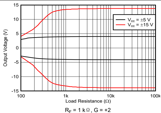
图 6-18. Output Voltage vs Differential Load Resistance
