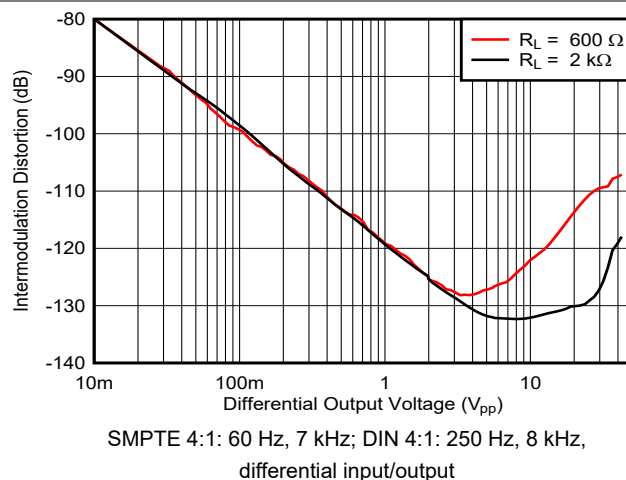
图 6-14. Intermodulation Distortion vs Output Voltage
