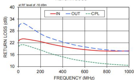
RETURN LOSS
