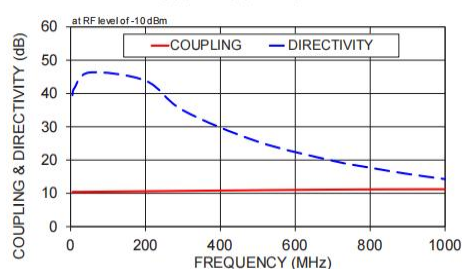
COUPLING & DIRECTIVITY
