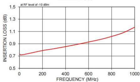
MAINLINE LOSS
