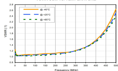
VSWR SUM vs. TEMPERATURE
